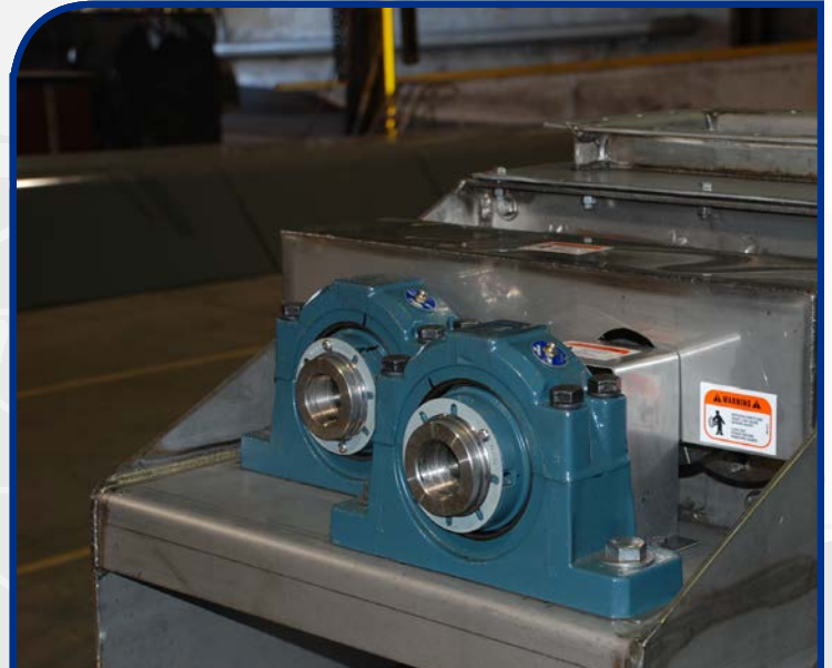
9" Twin Pedestals
