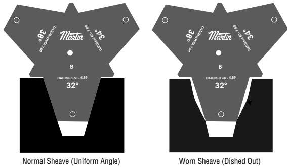
Normal Sheave (Uniform Angle)
