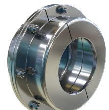
Vertical/Split Cover
