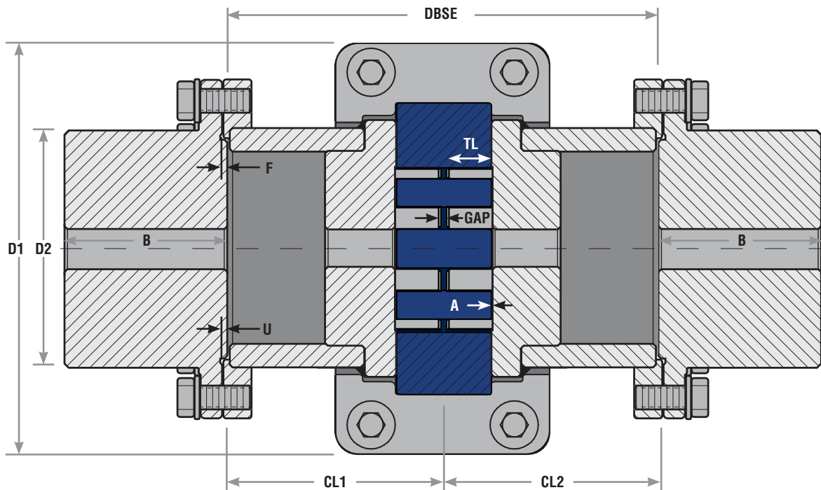
Martin Go-Flex® T31 Single Ended Full Spacer Coupling Dimensions/Ratings
