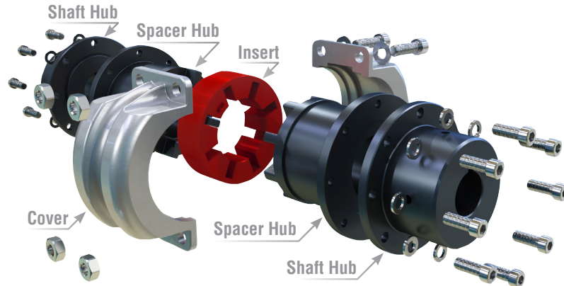
Single Ended Full Spacer Type T31 Application Shaft Separation DBSE (Distance Between Shaft Ends)
