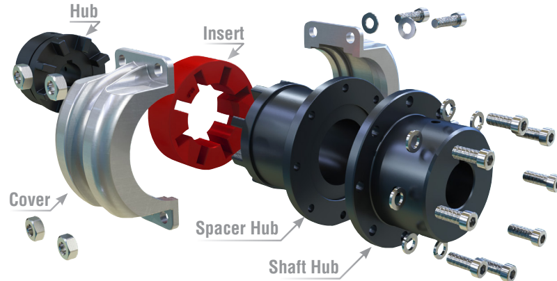
Single Ended Half Spacer Type T35 Application Shaft Separation DBSE (Distance Between Shaft Ends)
