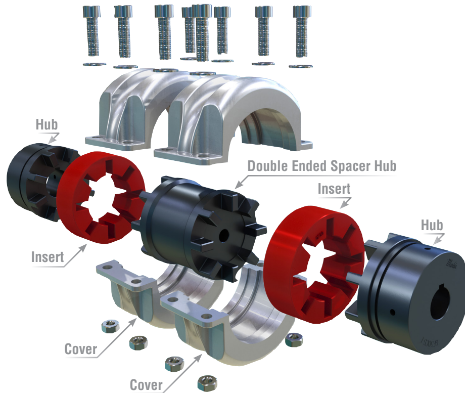
Double Ended Spacer Length Type T31 Application Shaft Separation - DBSE (Distance between Shaft Ends)
