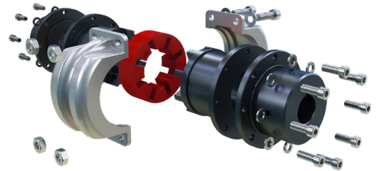
T31 – HS Cover Assembly
